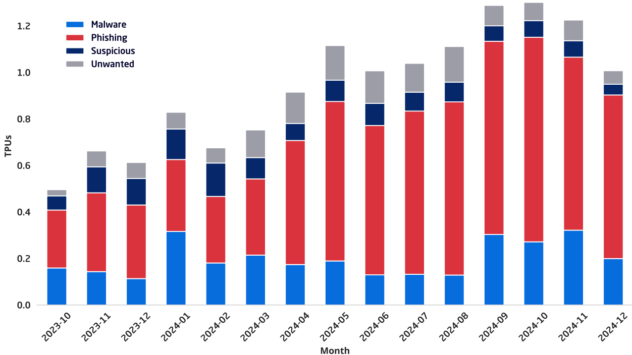
Chart 2b: Removing the overwhelming influence of the spam dataset shows that Phishing is on the rise, and a surge in Malware attacks late in the second half of 2024. In December 2024, malware detection in Sub-Saharan Africa surged by 42.14%, significantly higher than the previous year, driven by political instability and increased cyber activity. Additionally, the region is witnessing a rise in ransomware attacks, which are becoming more opportunistic, often exploiting vulnerabilities and delivered as secondary infections, indicating a concerning trend in the threat landscape.
